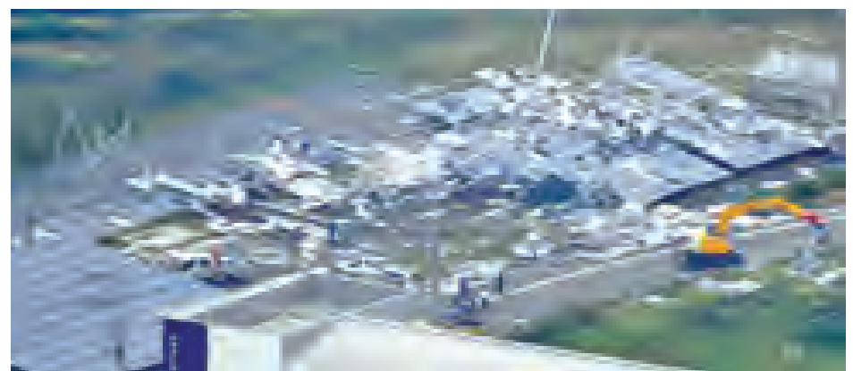
Photo taken from a Kyodo News helicopter shows solar panels destroyed by strong winds on 15 June, 2015, in the city of Isesaki, north of Tokyo. The winds overturned cars and damaged roofs in Isesaki and nearby areas.— KYODO NEWS
