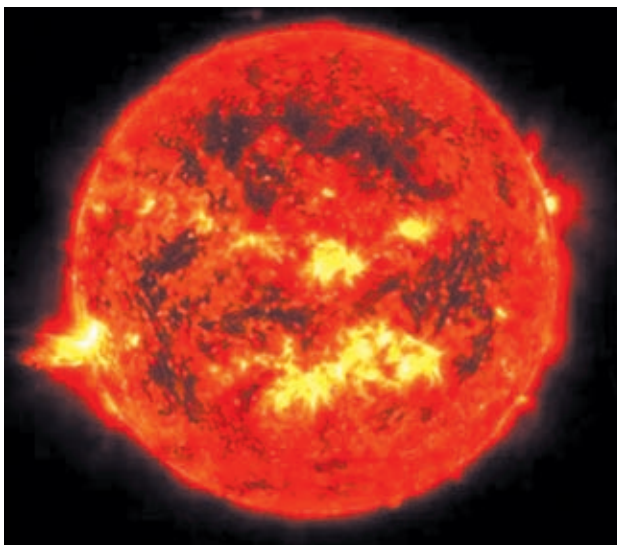
The bright light of a solar flare on the left side of the sun and an eruption of solar material shooting through the sun's atmosphere, called a prominence eruption, are seen in this NASA handout image taken June 20, 2013, at 11:15 pm EDT (03:15 GMT).—REUTERS
