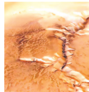
The High-Resolution Stereo Camera (HRSC) on board ESA's Mars Express has returned images of Echus Chasma, one of the largest water source regions on the Red Planet. REUTERS
