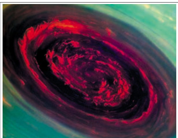
Saturn's hurricane
