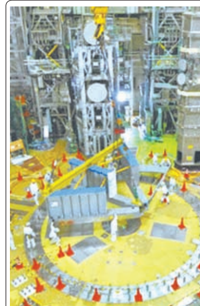
Photo taken on 28 Jan, 2013, shows the JT60SA, an experimental nuclear fusion device which the Japan Atomic Energy Agency and the European Union started assembling the same day, aiming at starting operation in 2019, at the agency's research facility in Naka, Ibaraki Prefecture. KYODO NEWS
