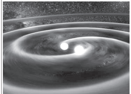
This is an artist's conception of J0651 with ripples to demonstrate how the white dwarf pair is emitting gravitational waves.
