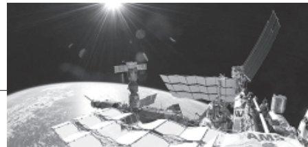
The experiment, seen here installed on the space station, cost some $2bn. INTERNET
