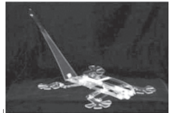
Despite its simple design, RightingBot rights itself in mid-air with a swing of its tail just like the lizards that inspired it.
