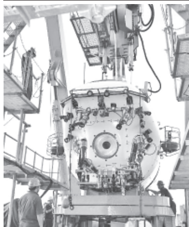
Photo taken on 22 June, 2012 shows the Jiaolong, China's manned deep-sea submersible, on the deck of the mother ship Xiangyanghong 09 in the Mariana Trench. The Jiaolong completed its third dive into the Mariana Trench and returned to the mother ship with a biological sample on Friday. The dive reached as deep as 6963 metres.—XINHUA
