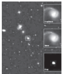
Galaxy CID-42 likely contains a massive black hole being ejected at several million miles per hour. The main panel is a wide-field optical image of CID-42 and the area around it.—INTERNET
