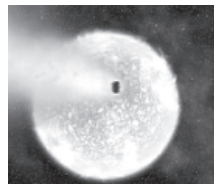
Artists' impression of "vanishing" planet.
