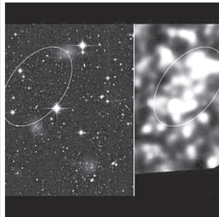
The Herschel Space Observatory has discovered a giant, galaxy-packed filament ablaze with billions of new stars.
