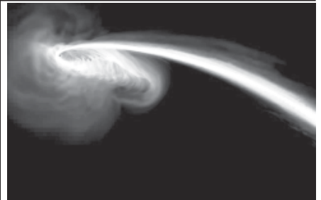
This computer-simulated image shows gas from a tidally shredded star falling into a black hole.
