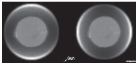
Polarised images of the red giant W Hydrae show the central star and a sphere of dust surrounding it.
