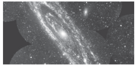
A mosaic view of the Andromeda galaxy created from 10 Galaxy Evolution Explorer images — INTERNET
