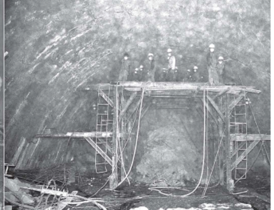
Vice-President Thiha Thura U Tin Aung Myint Oo inspects construction of spillway tunnel of Thahtay Hydropower Project.—MNA
