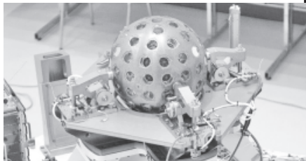
LARES will help scientists on the ground study the warping of space-time. — INTERNET
