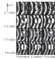
A near-field mapping of the disruption in the electric field distribution during the testing. Courtesy of The University of Texas at Austin.—INTERNET
