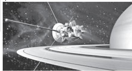
Artist concept of Cassini spacecraft.—INTERNET
