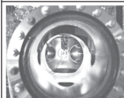
A small PETE device made with cesium-coated gallium nitride glows while being tested inside an ultra-high vacuum chamber.
