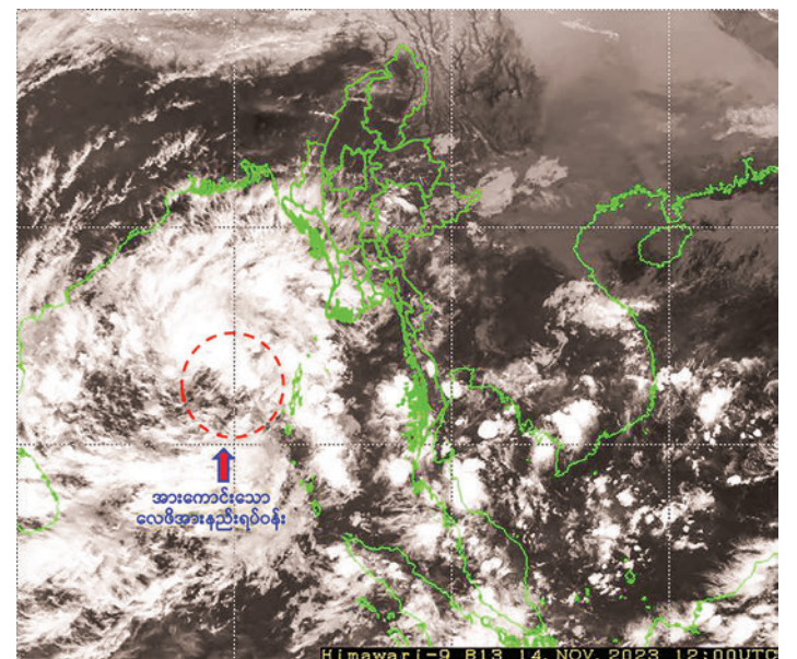
A satellite view of the well marked low pressure area.
