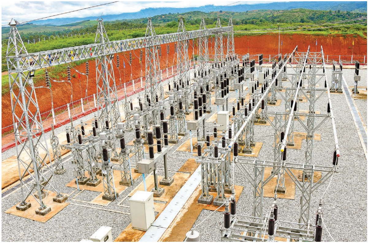
President U Win Myint inspects the Switchyard from the observation platform on the upper floor of Kengtung electrical substation on 8 August 2020. PHOTO:MNA
