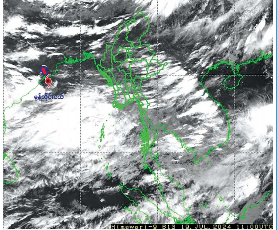
Himawari-9 B13 19. JUL. 2024 11:00UTC
