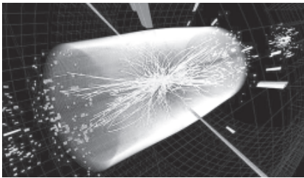
This document provided by European Organization for Nuclear Research (CERN) in Geneva shows a graphic showing traces of two high-energy photons measured in the Compact Muon Solenoid (CMS) experiment.
