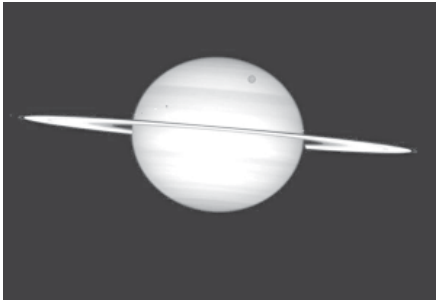
The NASA/ESA Hubble Space Telescope captured a photo sequence of four moons of Saturn passing in front of their parent planet. The moons, from far left to right, are the white icy moons Enceladus and Dione, the large orange moon Titan, and icy Mimas. Due to the angle of the Sun, they are each preceded by their own shadow.—INTERNET
