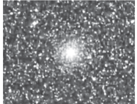
Bright, young pulsar spotted by Fermi.
