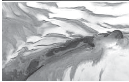
This image was acquired by the Mars Express High-Resolution Stereo Camera on 17 May 2010 and shows a part of the northern polar region of Mars at the northern hemisphere summer solstice. INTERNET
