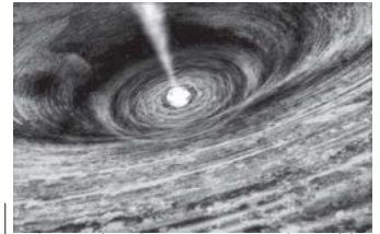
This undated artistic view released by the NASA shows a close-up of a supermassive black hole.—INTERNET
