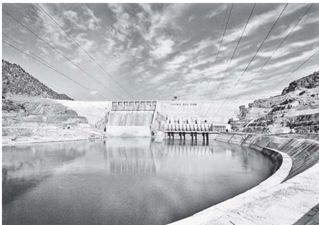
The RCC dam and the outfall channel of the plant.
