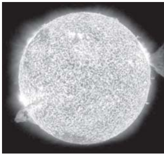
This image of the sun, captured by The Solar Dynamics Observatory spacecraft 28 January, 2011, shows nearly simultaneous solar eruptions on opposite sides of the Sun, in this photograph released by NASA 28 January.—XINHUA
