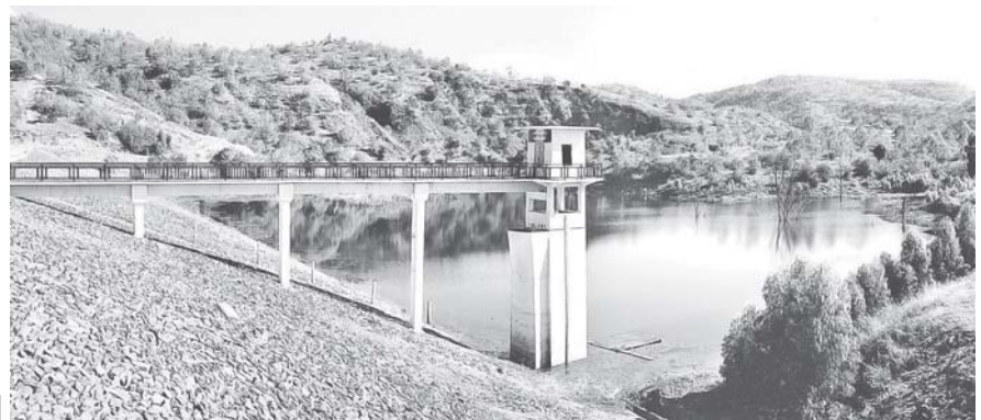
Photo shows Bawditahtaung Dam.
