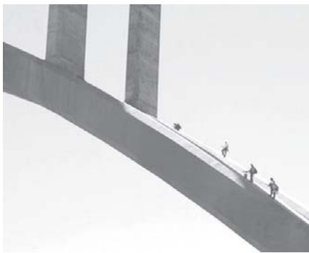
In this photo taken on 26 April, 2010, construction workers use climbing equipment as they work on the Hoover Dam Bypass over the Colorado River. Completion is expected late 2010 and will result in a bridge spanning 900 feet above the Colorado River between Arizona and Nevada.
