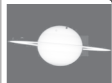
An image of four moons of Saturn passing in front of their parent planet in seen this image taken by NASA's Hubble Space Telescope 24 February, 2009 and released by NASA 17 March, 2009.
