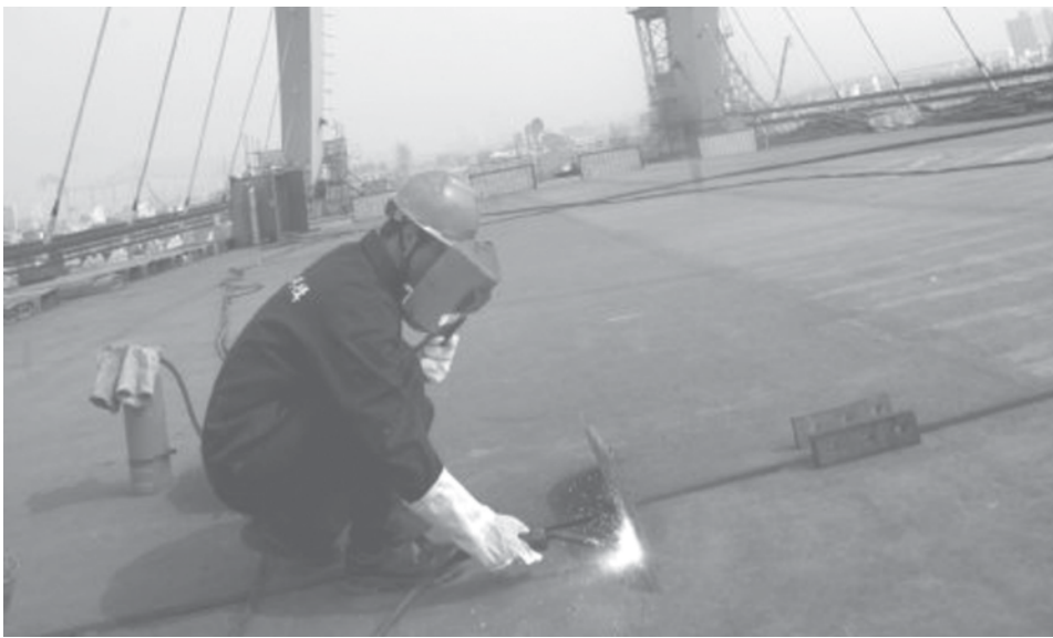
A worker welds the last box girder for the Chuanyang River Bridge, a "VIP bridge" for the 2010 World Expo, in east China's Shanghai Municipality on 29 Aug, 2009. Crossing the Chuanyang River, the bridge joined its two sections after four months' construction on Saturday and would serve as a way leading the VIPs directly to the Shanghai Expo Park through VIP thoroughfare.—XINHUA
