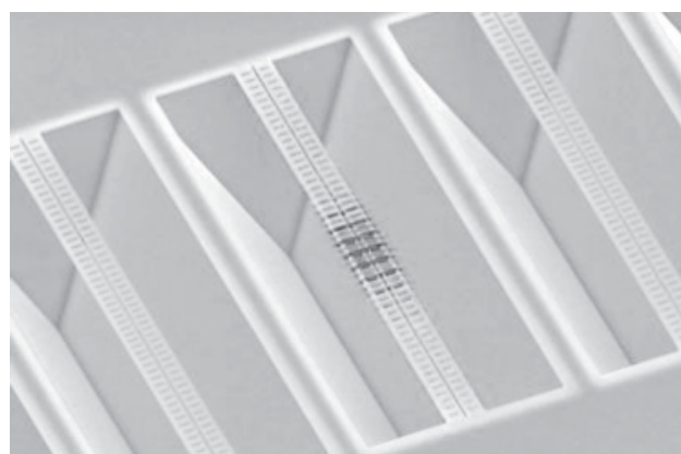
Scanning electron microscope image of an array of "zipper" optomechanical cavities. The scale and sensitivity of the device is set by its physical mass (40 picograms/40 trillionths of a gram) and the nanoscale gap between the two nanobeams.
