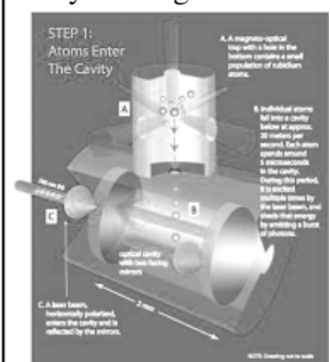
Step one in single-atom detection system.
