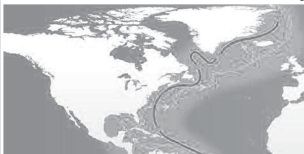
This model of North Atlantic currents has been called into question by new data from Duke University and the Woods Hole Oceanographic Institution.
