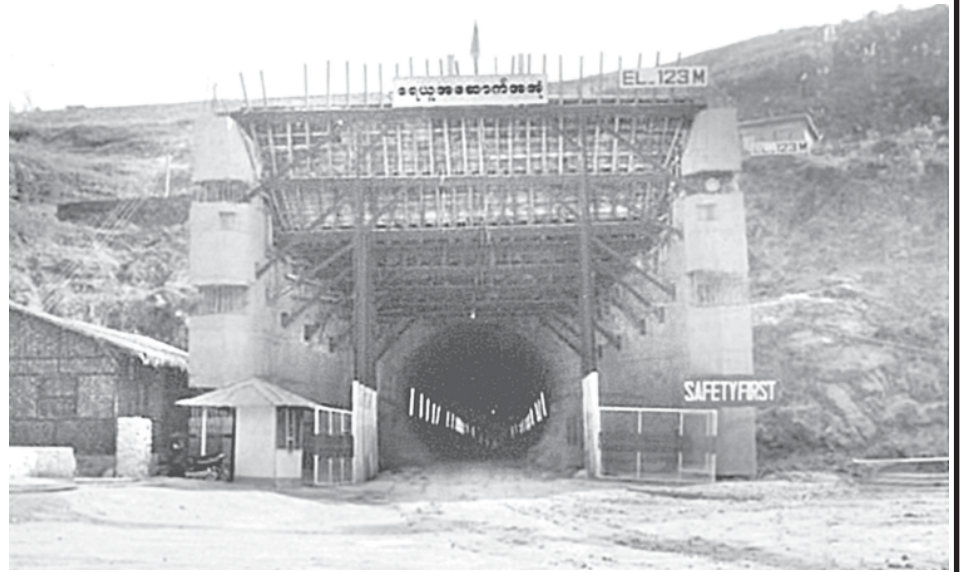
Photo shows progress of concrete work at power intake structure of Pyuchaung Hydropower Project on 30 March 2009.
