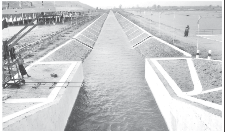
Water flowing in 29.72 miles long left main canal of Paunglaung Diversion Weir to irrigate 16,000 acres of farmlands.
