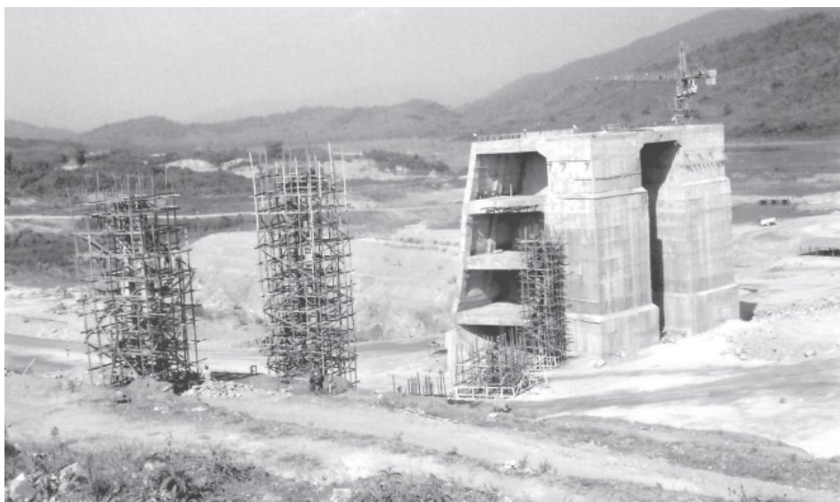
The intake structure and bridge will be parts of Shwegyin Hydropower Plant.
