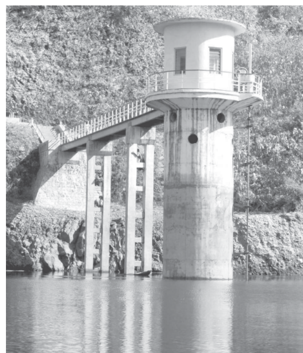
Control tower of Pyaingchaung Dam seen with embankment in the background.
