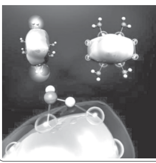
The figure shows aluminum clusters reacting with water to produce hydrogen.
