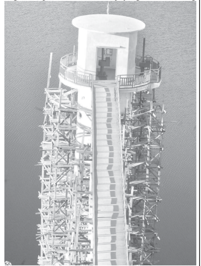
The control tower under construction of Zeechaung Dam.
