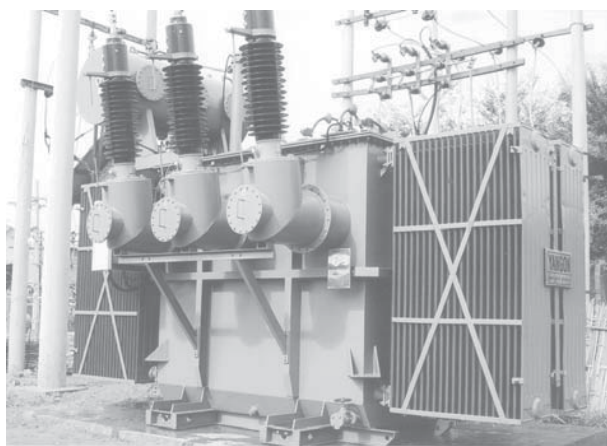
66/11 KV 10000 KVA Yangon Transformer installed at Lawkananda River Water Pumping Project.
