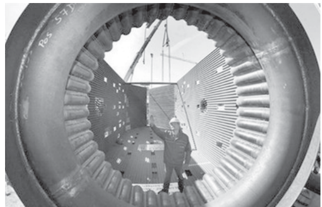
Vattenfall’s CO2-free power plant in the eastern German town of Schwarze Pumpe. —INTERNET
