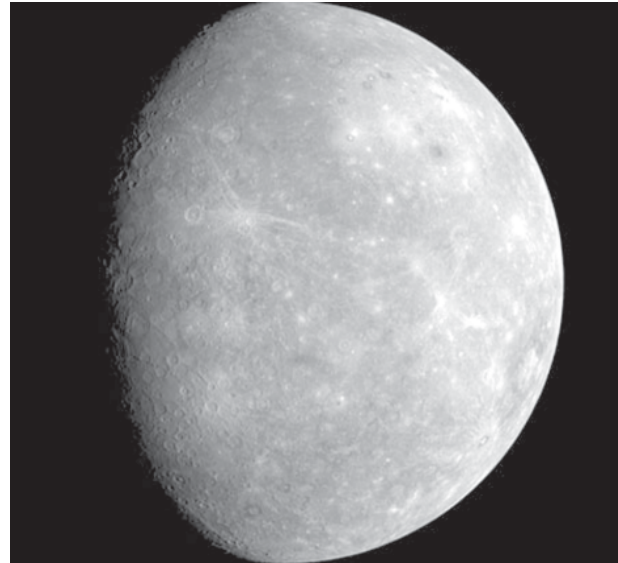
An image of Mercury is seen as taken by NASA's Messenger spacecraft at a distance of approximately 17,000 miles (27,359 km) after the spacecraft's closest approach to the planet on 15 Jan, 2008.—INTERNET
