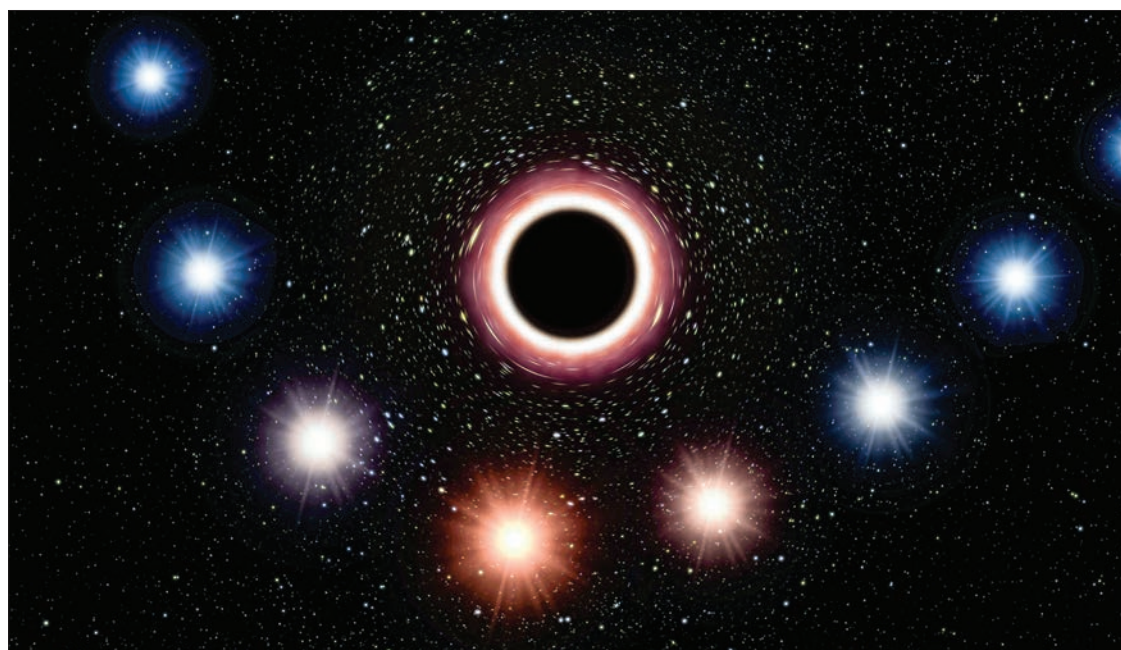
A handout photo released on July 26, 2018 by the European Southern Observatory shows an artist impression of the path of the star S2 as it passes very close to the supermassive black hole at the centre of the Milky Way. As it gets close to the black hole the very strong gravitational field causes the colour of the star to shift slightly to the red, an effect predicted under Einstein's general theory of relativity. In this graphic the colour effect and size of the objects have been exaggerated for clarity. PHOTO: AFP
