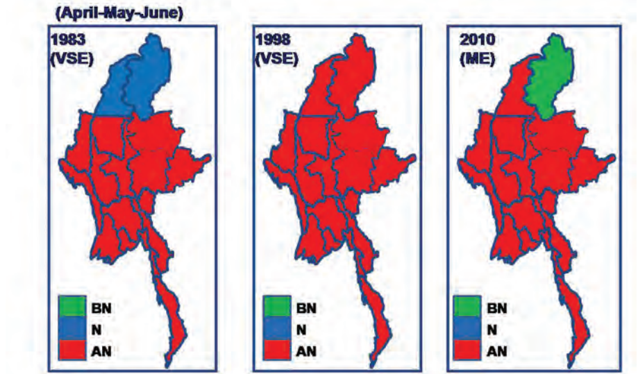
Historical Data of Seasonal Observed Maximum Temperature (°C) Conditioned on Specific El-Nino Years (Source: DMH Data)
