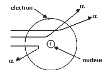
Fig. Scattering of alpha particle
