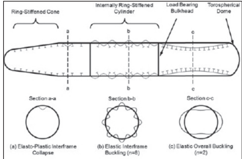
Figure 2: Typical pressure hull structure and buckling modes
